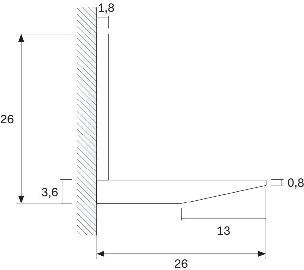
Con schiena With back panel
