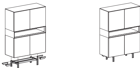
Esploso del basamento Exploded view of the base
